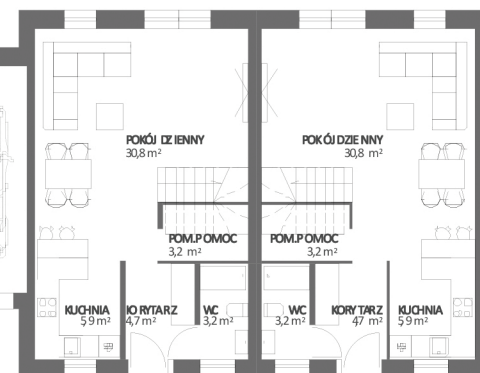
PARTER SEGMENT L+G PARTER SEGMENT P
