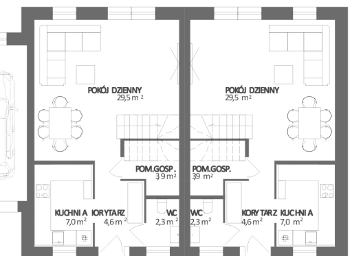
PARTER SEGMENT L+G PARTER SEGMENT P
