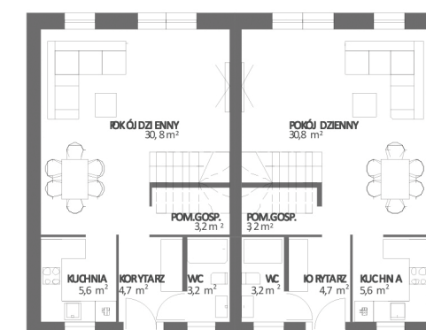
PARTER SEGMENT L PARTER SEGMENT P+G
